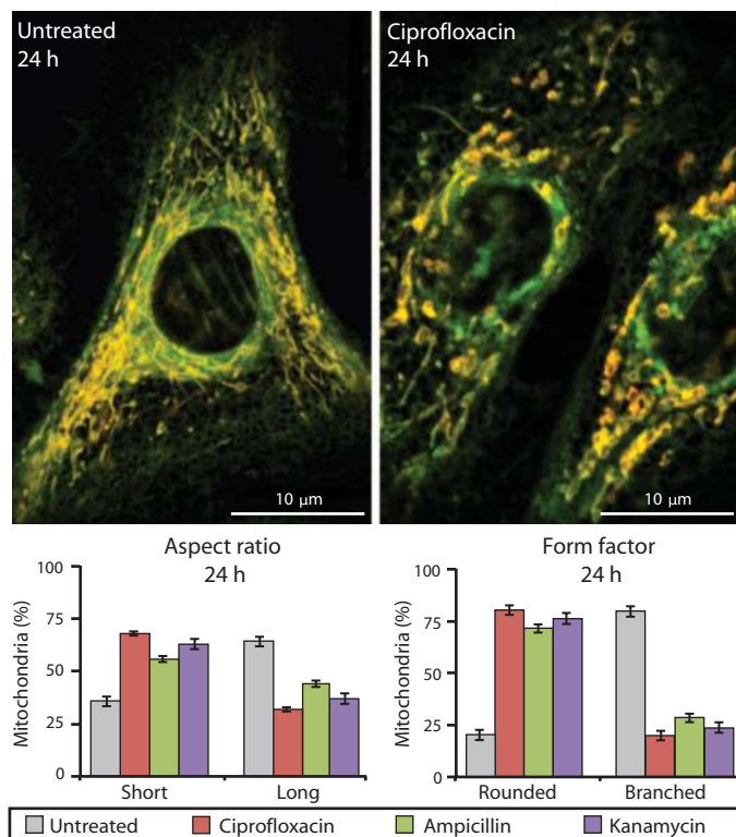
Fig. 3. Mitochondria in bactericidal antibiotic-treated cells show an abnormal, proflission state. Mitochondrial morphology was measured in primary human mammary epithelial cells using TMRE and MitoTracker Green. Untreated samples (left image) show mitochondria with normal morphology, which are long and highly branched. Ciprofloxacin-treated cells (10 \mu\text{g/ml} ) (right image) had abnormally short and truncated mitochondria. The percentages of mitochondria with a short versus long aspect ratio and rounded versus branched form factor were measured for untreated and bactericidal antibiotic-treated cells. Data are means \pm SEM ( n \geq 5 ).
